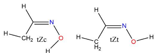
Figure 10. Acetaloximes, Z .
